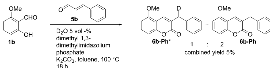
Scheme 4. Reaction between 1b and 5b in the presence of 5 vol.-% D_2O .
