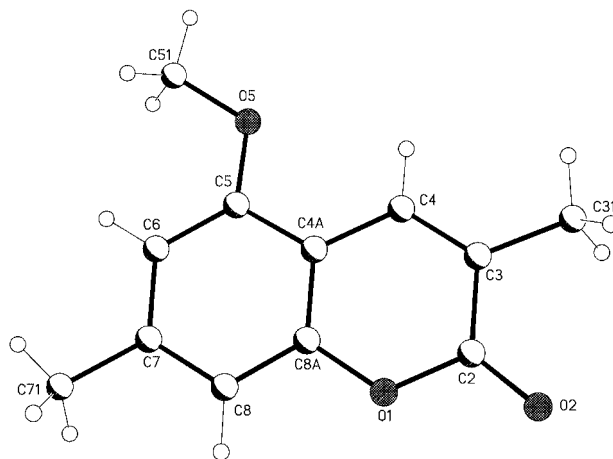
Figure 1. X-ray structure of 6d-H .
