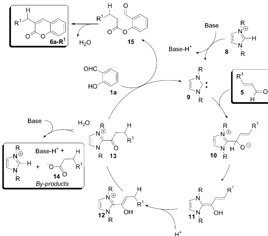
Scheme 3. Mechanism for formation of coumarin 6a from \alpha,\beta -unsaturated aldehydes and salicylaldehydes via NHCs.
