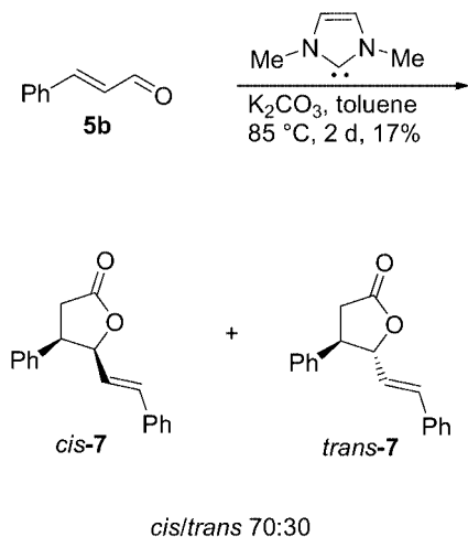
Scheme 2. Synthesis of \gamma -butyrolactones 7 from cinnamaldehyde in dimethyl 1,3-dimethylimidazolium phosphate and toluene.
