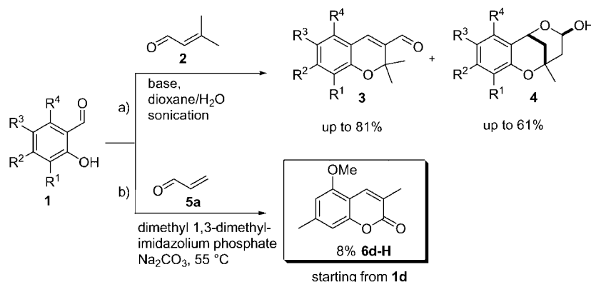
Scheme 1. Reaction path a : synthesis of 2,2-dimethyl-2H-chromene-3-carbaldehydes 3 and 9-methyl-8,12-dioxatricyclo[7.3.1.0 2,7 ]trideca-2,4,6-trien-11-ols 4 . [15] Reaction path b : preliminary synthesis of coumarin 6d-H .
